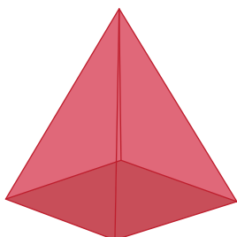
Square pyramid
