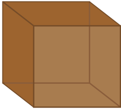
Cube
