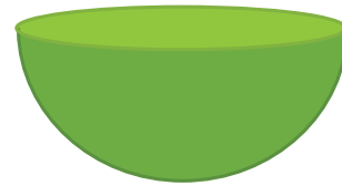
Hemisphere
