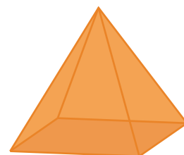
Rectangular pyramid
