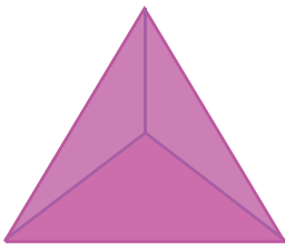
Triangular pyramid
