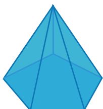
Pentagonal pyramid
