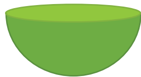
Hemisphere
