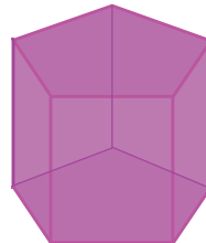
Pentagonal prism
