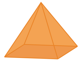
Rectangular pyramid
