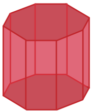
Octagonal prism
