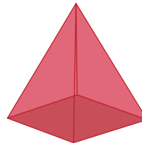
Square pyramid
